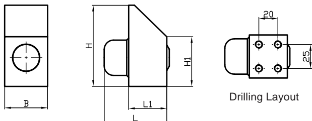
Bolt Contact Modules 1/2 Fold
