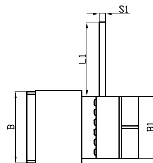
Special Version with 90° angled connection plate
