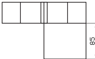
contact block with one connecting tab Part.-No. 50139 50141
