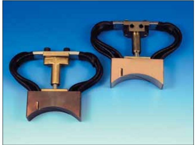
High Current Carbon Brushes with Combination Holders
