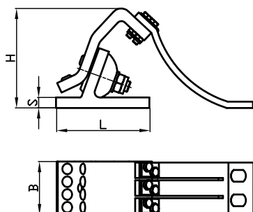
Part No. 51295 2 Piece Standard Version
