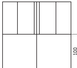
contact block with double connecting tab Part.-No. 50143 50161 50146 50166 50151 50171 50156 50176
